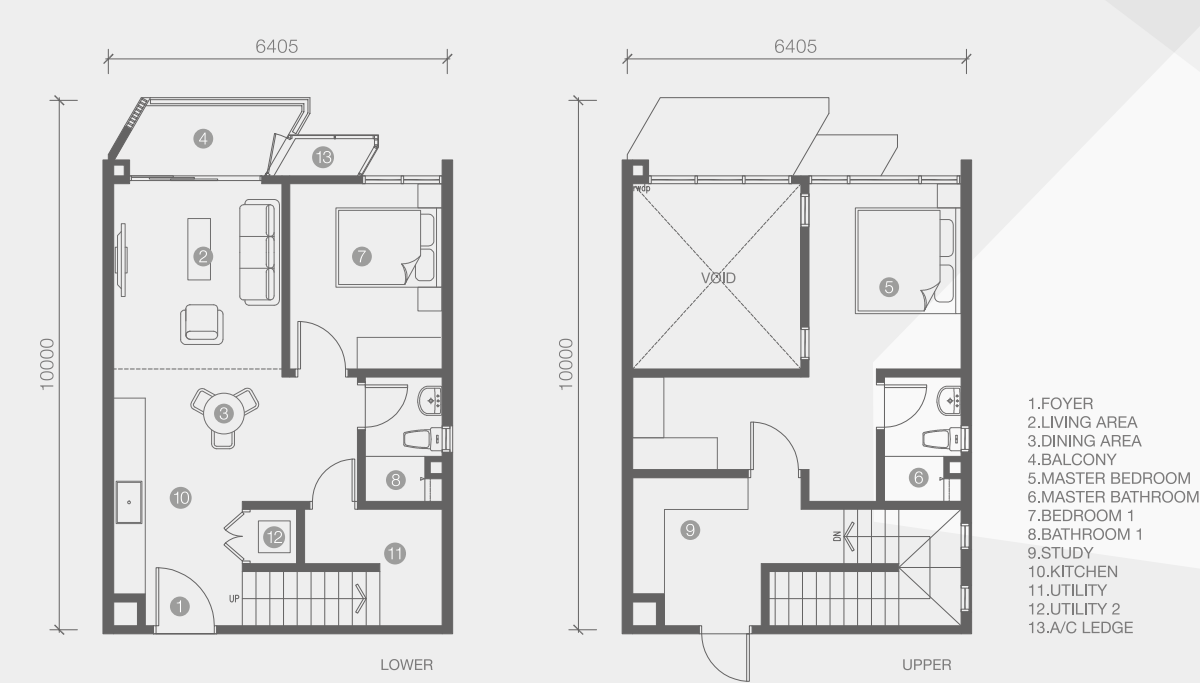
Type B1 1105 SQ.FT. 2 Bedrooms + 2 Utilities + 1 Study
