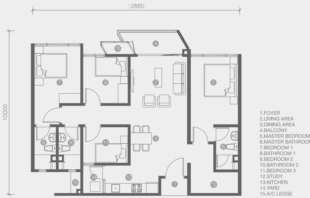
Type A3 1205 SQ.FT. 4 Bedrooms + 1 Study
